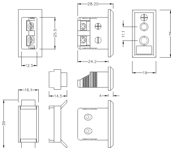
Standard Fascia Socket (with nylon mounting clip)
