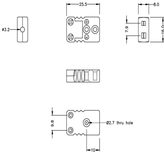
Miniature Hi-Temp Plastic in-line Socket - HTP (dimensions in mm)
