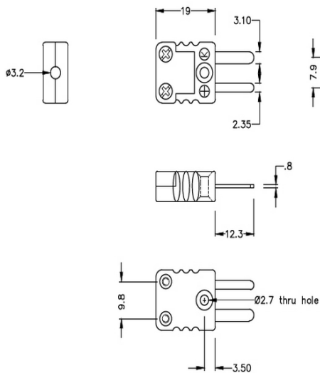
Miniature Hi-Temp Plastic in-line Plug - HTP (dimensions in mm)
